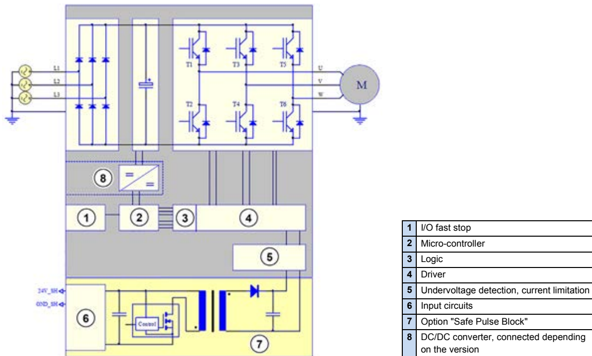
Figure 1: Structure of Safe Pulse Block
