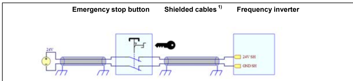
1) Shielded cables to exclude faults as per DIN EN ISO 13849-2
