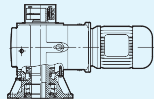
SK 90...1 AFSH VL2 mm \Rightarrow D117 SK 90...1 AFSH VL3 \Leftarrow
