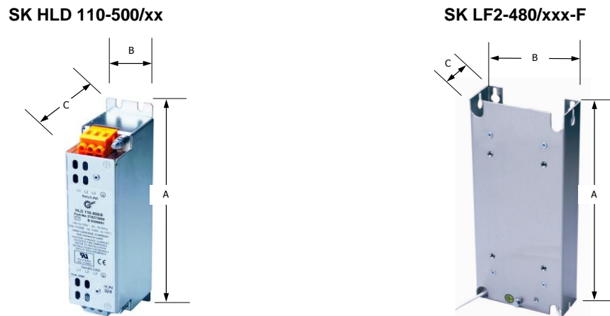
Figure 18: Dimensions of chassis and footprint mains filters SK HLD 110-500/xx and SK LF2-480/xxx-F
