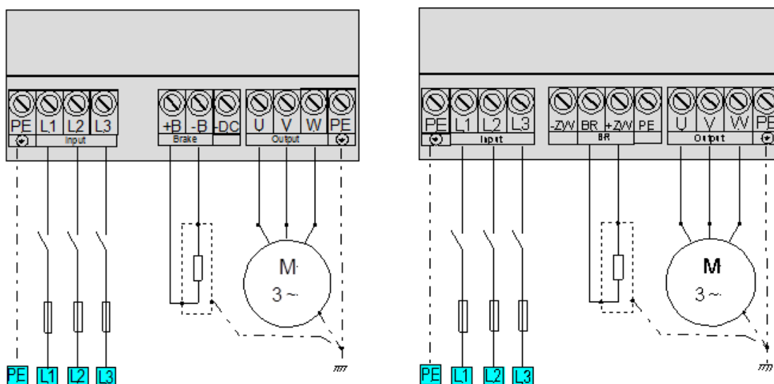
Figure 9: Power connection SK 700E
