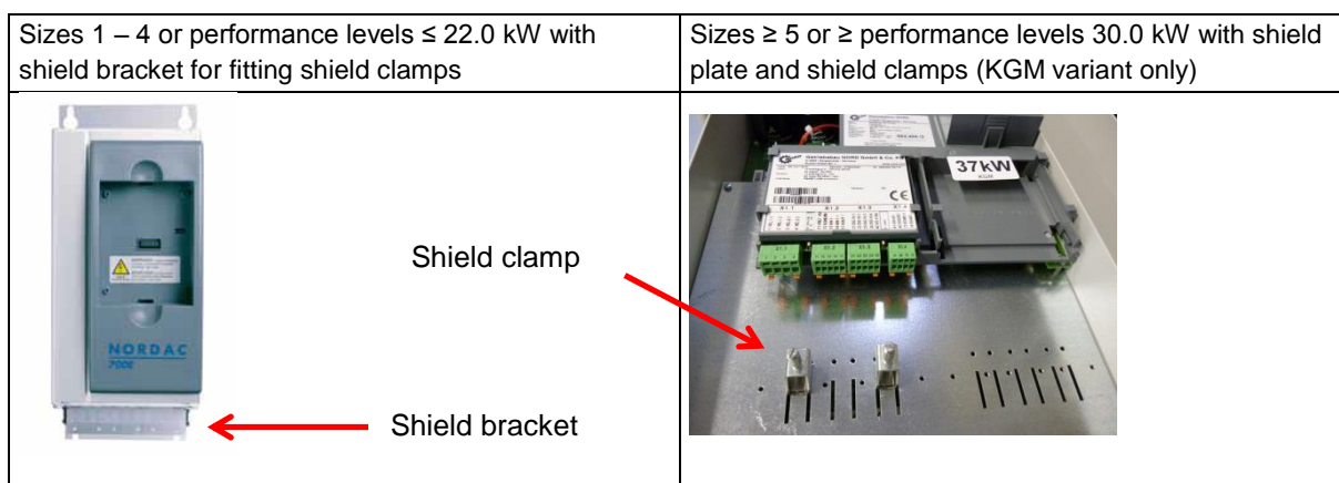
Figure 3: SK 700E: different types (with shield bracket or shield plate)
