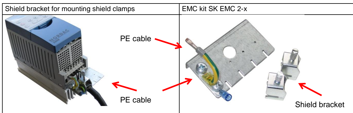
Figure 4: SK 5xxE size-dependent EMC kits (with shield bracket, shield clamps, PE cable)
